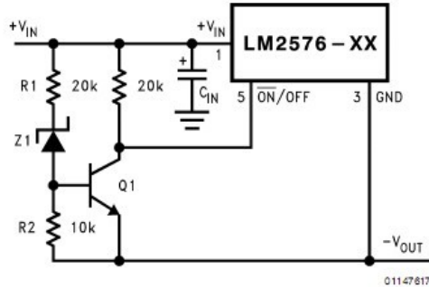
FIGURE 13. Undervoltage Lockout for Buck-Boost Circuit
