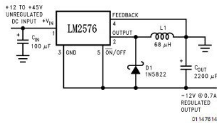
FIGURE 10. Inverting Buck-Boost Develops -12V
