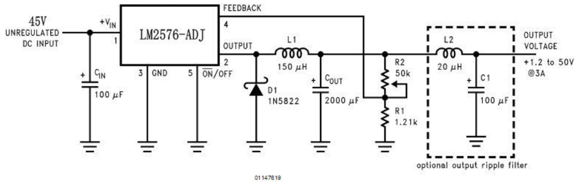
FIGURE 15. 1.2V to 37V Adjustable 3A Power Supply with Low Output Ripple
