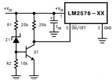
FIGURE 12. Undervoltage Lockout for Buck Circuit
