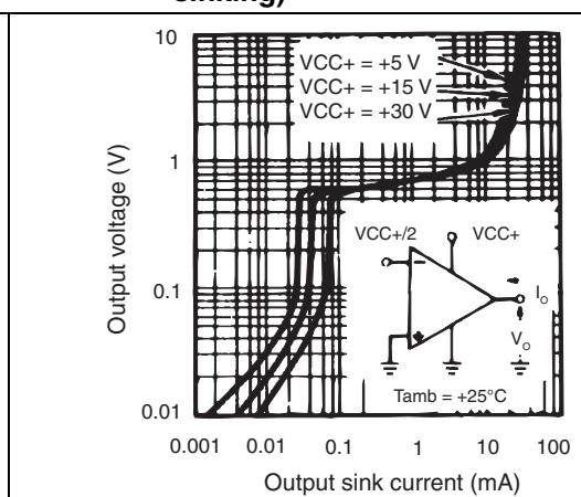
Figure 12. Output characteristics (current sinking)
