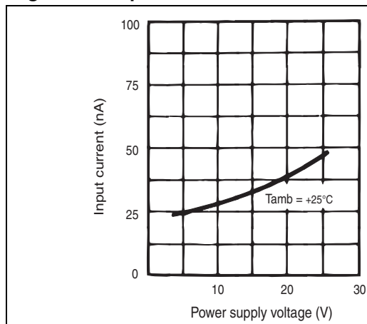
Figure 15. Input current
