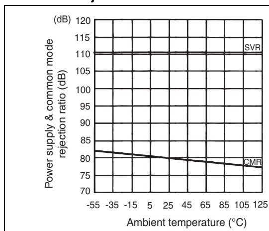
Figure 17. Power supply and common mode rejection ratio
