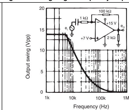
Figure 10. Large signal frequency response
