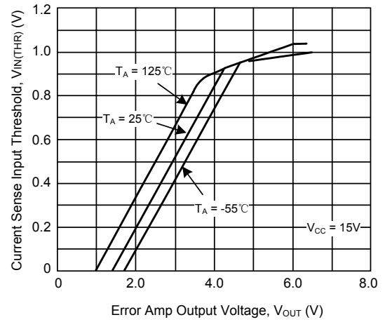
Current Sense Input Threshold vs. Error Amp Output Voltage
