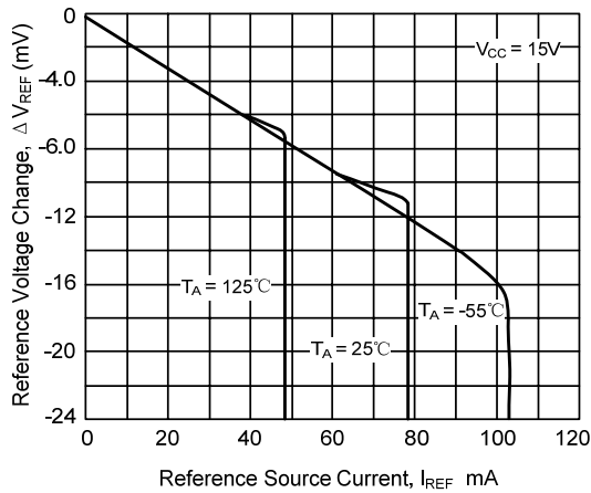
Reference Voltage Change vs. Reference Source Current
